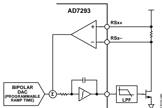
Figure 46. Closed-Loop Control
