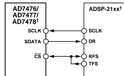
Figure 27. Interfacing to the ADSP-21xx
