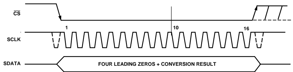
Figure 19. Normal Mode
