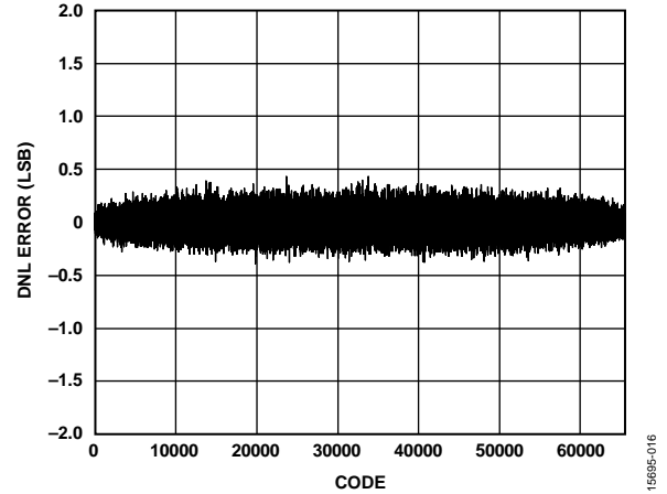
Figure 16. Typical DNL Error, \pm 5 V Range
