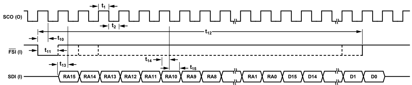
Figure 3. Register Write Timing Diagram
