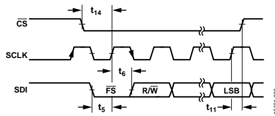
Figure 3. SPI Write Timing Diagram
