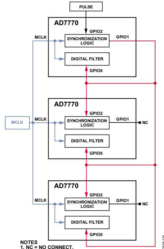
Figure 110. Hardware ODR Update
