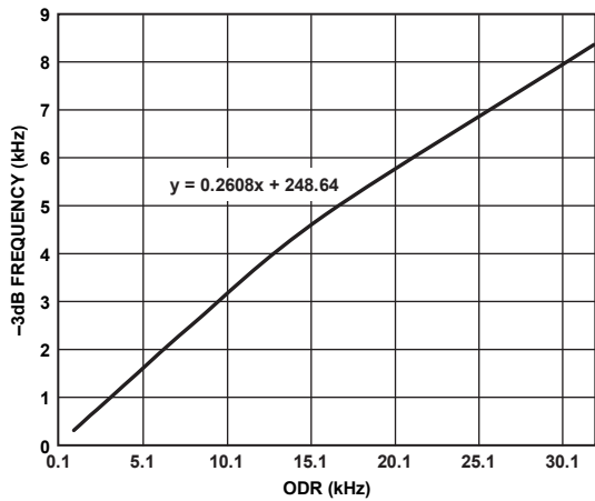
Figure 112. -3 dB Correction Factor
