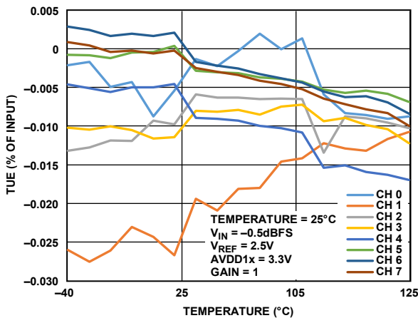
Figure 52. Total Unadjusted Error (TUE) vs. Temperature, High Resolution Mode
