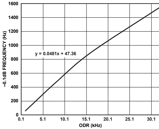
Figure 111. -0.1 dB Correction Factor
