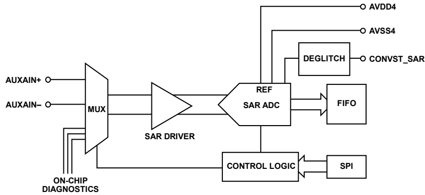
Figure 107. SAR ADC Configuration and Control
