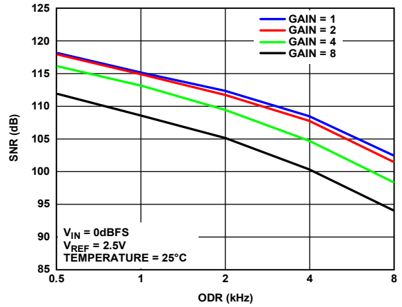
Figure 41. SNR vs. ODR at 4 kSPS, Low Power Mode
