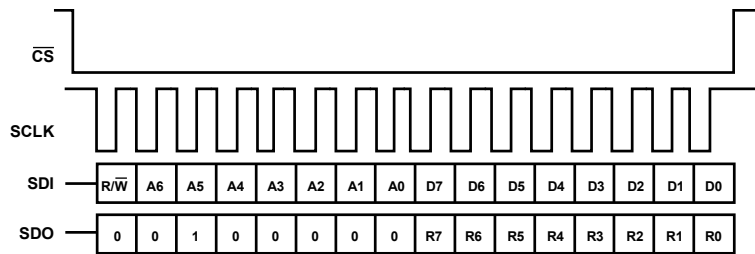
Figure 102. 16-Bit SPI Transfer—CRC Disabled
