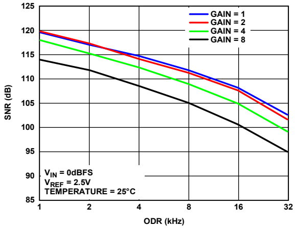
Figure 38. SNR vs. ODR at 16 kSPS, High Resolution Mode
