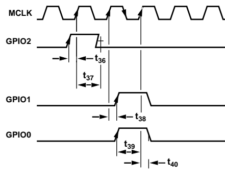
Figure 6. GPIOs for SRC Update Timing Diagram
