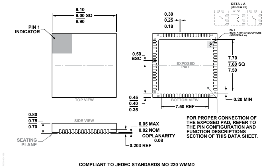
COMPLIANT TO JEDEC STANDARDS MO-220-WMMD Figure 122. 64-Lead Lead Frame Chip Scale Package [LFCSP] 9 mm × 9 mm Body and 0.75 mm Package Height (CP-64-15) Dimensions shown in millimeters
