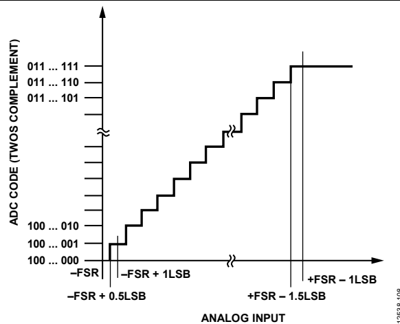
Figure 91. Transfer Function
