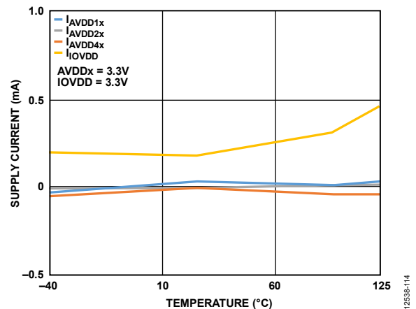
Figure 97. Shutdown Current
