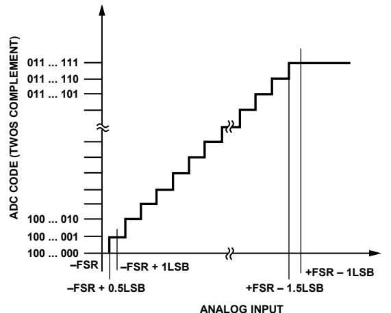
Figure 90. Transfer Function
