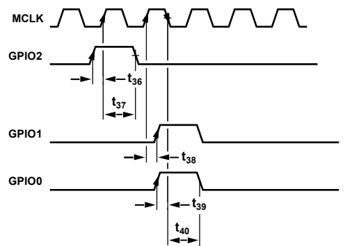
Figure 6. GPIOs for SRC Update Timing Diagram
