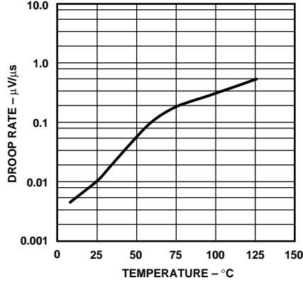
Droop Rate vs. Temperature, V_{IN} = 0\text{ V}
