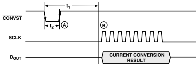
Figure 14. Mode 1 Operation Timing
