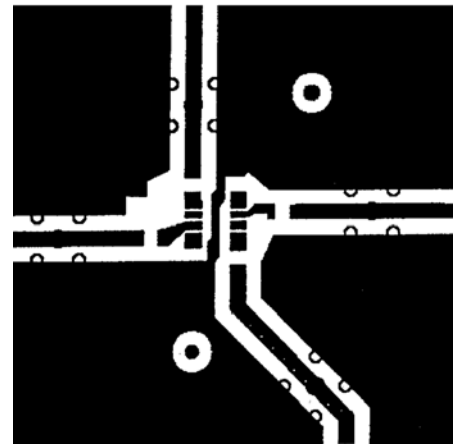
Figure 65. Noninverter SOIC Board Layout (Component Layer)
