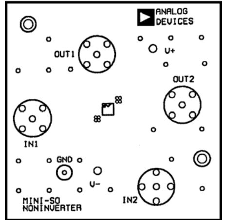
Figure 63. Noninverter MSOP Board Layout (Silkscreen)
