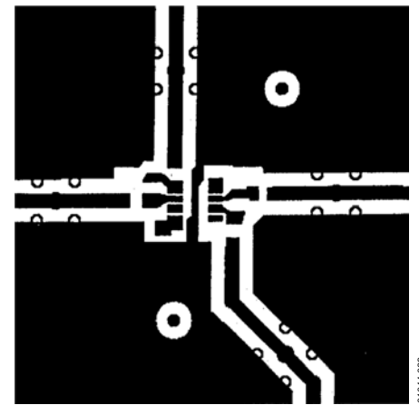
Figure 64. Inverter SOIC Board Layout (Component Layer)
