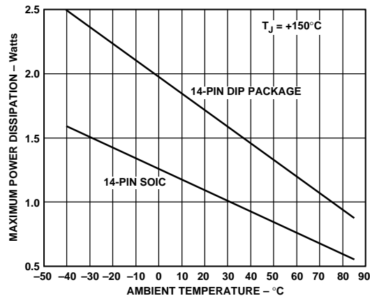
Maximum Power Dissipation vs. Ambient Temperature
