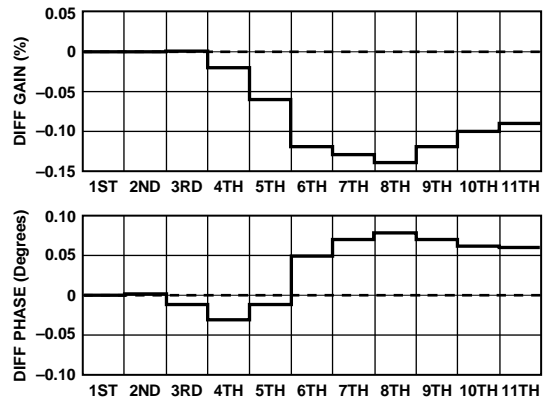
Figure 24. Differential Gain and Phase @ V S = ±5V; R L = 1 kΩ
