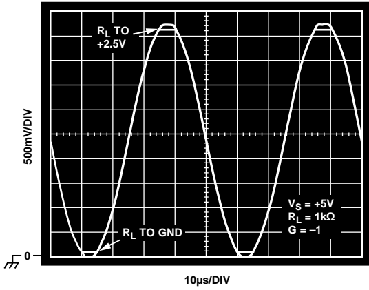
Figure 38. Output Swing
