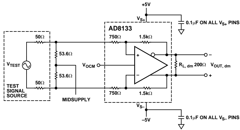
Figure 33. Basic Test Circuit
