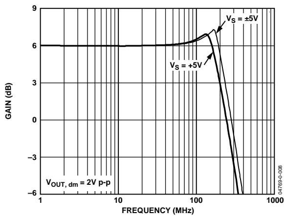
Figure 6. Large Signal Frequency Response for Various Power Supplies
