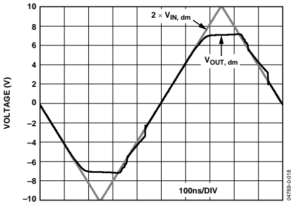
Figure 13. Overdrive Recovery
