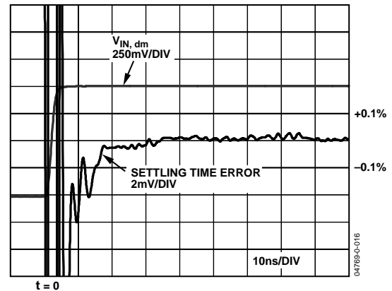
Figure 16. Settling Time (0.1%)
