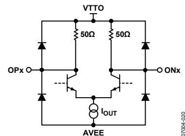
Figure 20. High Speed Output Simplified Schematic
