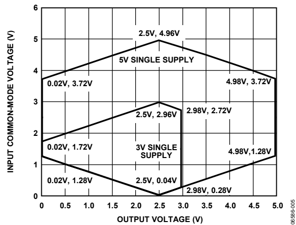
Figure 14. Instrumentation Amplifier Input Common-Mode Range vs. Output Voltage, All Gains, V_{REF} = 2.5V
