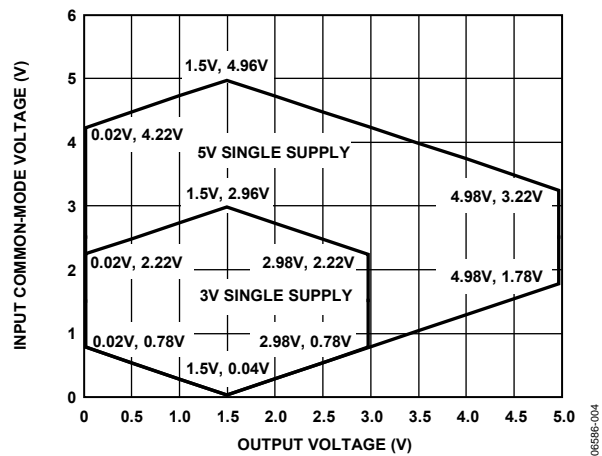
Figure 13. Instrumentation Amplifier Input Common-Mode Range vs. Output Voltage, All Gains, V_{REF} = 1.5V
