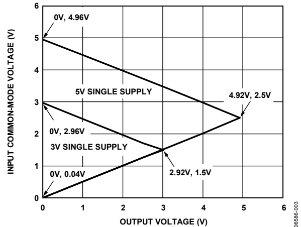
Figure 12. Instrumentation Amplifier Input Common-Mode Range vs. Output Voltage, All Gains, V_{REF} = 0V
