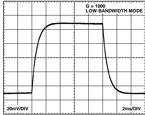
Figure 49. Small Signal Pulse Response, G = 1000 , R_L = 10\text{ k}\Omega , C_L = 100\text{ pF} , Low Bandwidth Mode
