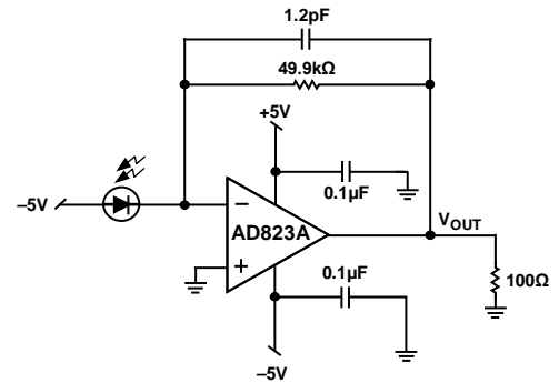
Figure 44. Photodiode Preamplifier
