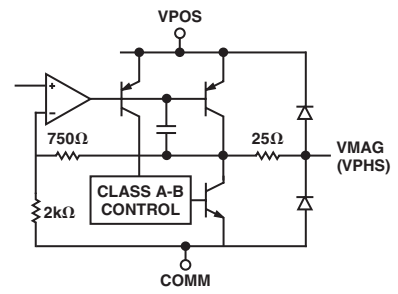
Circuit B
