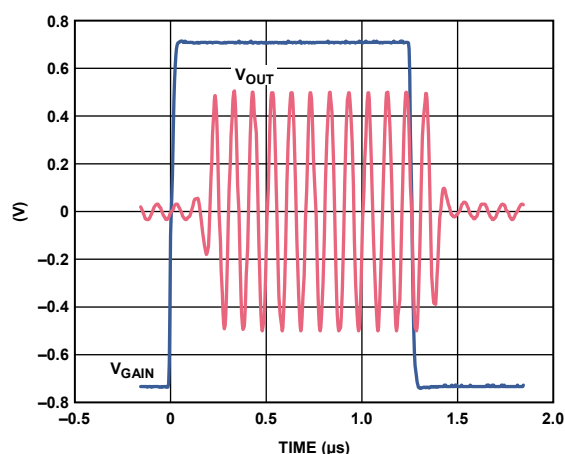
Figure 38. Gain Response (See Figure 54)
