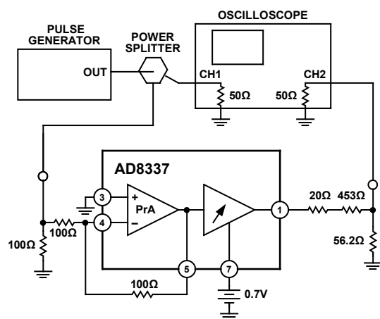
Figure 59. Pulse Response—Inverting Feedback
