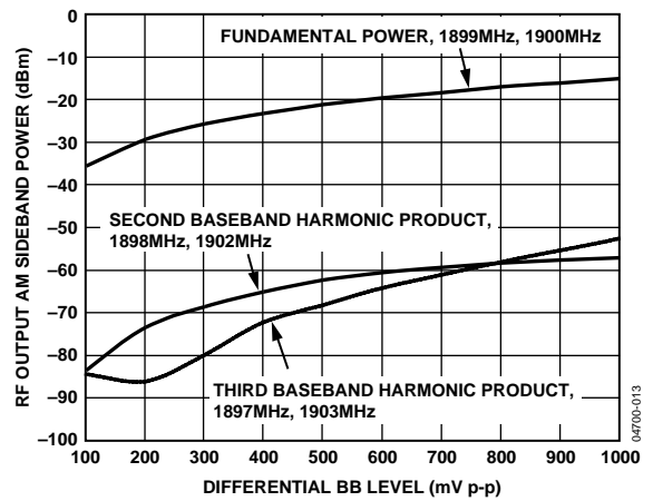
Figure 13. Baseband Harmonic Distortion (I and Q Channel, RF Input = 0 \text{ dBm} , Output Balun and Cable Losses of Approximately 2 \text{ dB} Not Accounted for in Plot)
