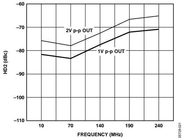
Figure 28. Single-Ended, Second-Order Harmonic Distortion (HD2) vs. Frequency, 200 \Omega Load
