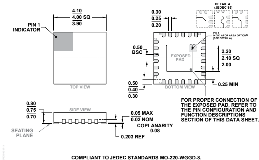
Figure 51. 24-Lead Lead Frame Chip Scale Package [LFCSPP] 4 mm × 4 mm Body and 0.75 mm Package Height (CP-24-10) Dimensions shown in millimeters
