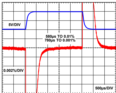
Figure 50. Large Signal Pulse Response and Settling Time, 10 V Step, Dual Supply, V_S = \pm 15 V , G = 1000
