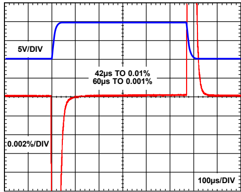
Figure 49. Large Signal Pulse Response and Settling Time, 10 V Step, Dual Supply, V_S = \pm 15 V , G = 100
