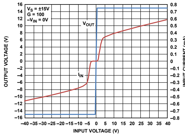
Figure 20. Input Overvoltage Performance, Dual Supply, V_S = \pm 15V , G = 100
