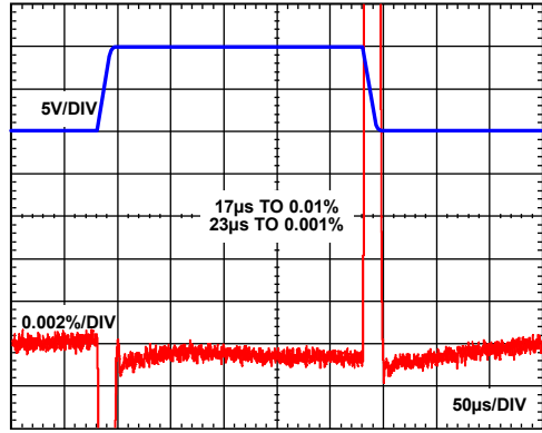
Figure 48. Large Signal Pulse Response and Settling Time, 10 V Step, Dual Supply, V_S = \pm 15 V , G = 10
