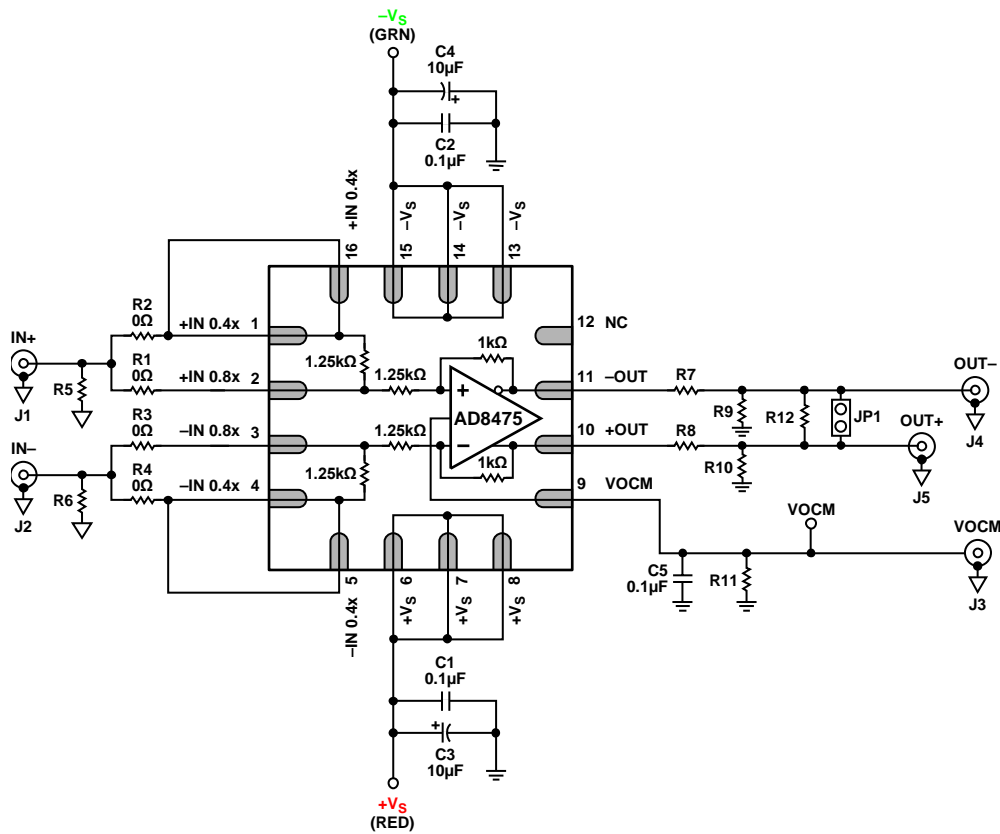
Figure 56. AD8475-EVALZ Schematic
