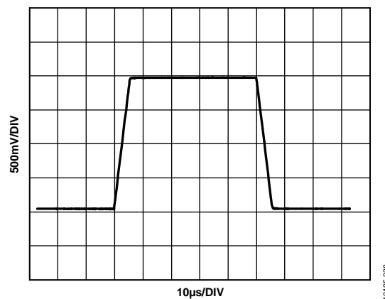
Figure 34. VOVM Large Signal Step Response
