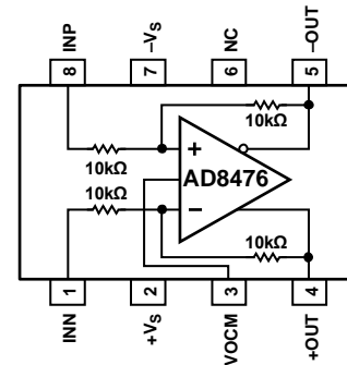
Figure 1. 8-Lead MSOP
