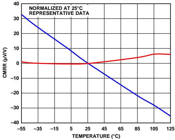
Figure 4. CMRR vs. Temperature, V_{CM} = \pm 20\text{ V}
