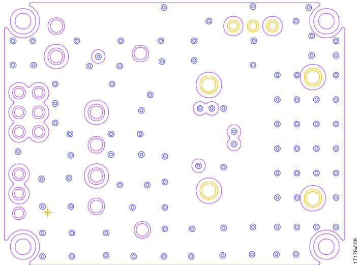
Figure 8. Evaluation Board Layout, Ground Plane (Layer 2)
