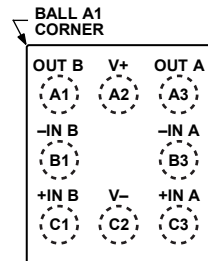
Figure 2. 6-Ball WLCSP (CB-6-7)
