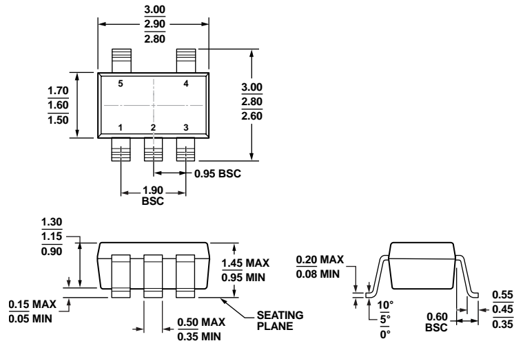
COMPLIANT TO JEDEC STANDARDS MO-178-AA Figure 40. 5-Lead Small Outline Transistor Package [SOT-23] (RJ-5) Dimensions shown in millimeters
