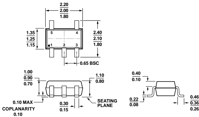
COMPLIANT TO JEDEC STANDARDS MO-203-AA Figure 41. 5-Lead Thin Shrink Small Outline Transistor Package [SC70] (KS-5) Dimensions shown in millimeters
