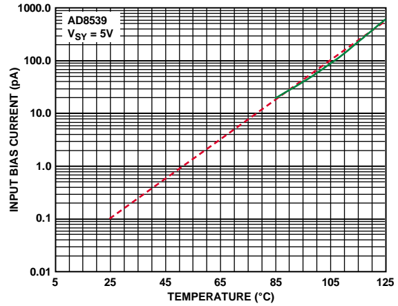
Figure 37. AD8539 Input Bias Current vs. Temperature
