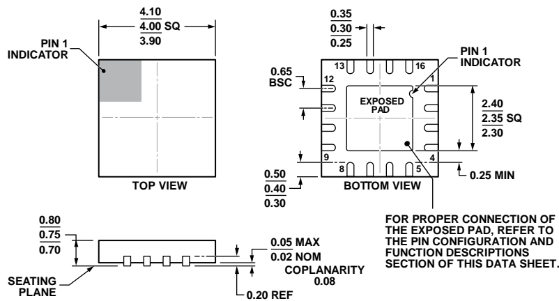
Figure 64. 16-Lead Lead Frame Chip Scale Package [LFCSP_WQ] 4 mm x 4 mm Body, Very Very Thin Quad (CP-16-20)
