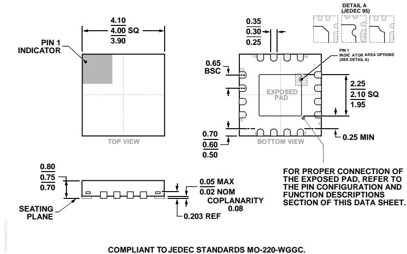
COMPLIANT TO JEDEC STANDARDS MO-220-WGGC. Figure 37. 16-Lead Lead Frame Chip Scale Package [LFCSP] 4 mm x 4 mm Body and 0.75 mm Package Height (CP-16-23) Dimensions shown in millimeters
