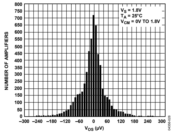
Figure 28. V_{OS} Distribution
