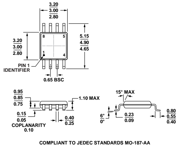
Figure 68. 8-Lead Mini Small Outline Package [MSOP] (RM-8) Dimensions shown in millimeters
