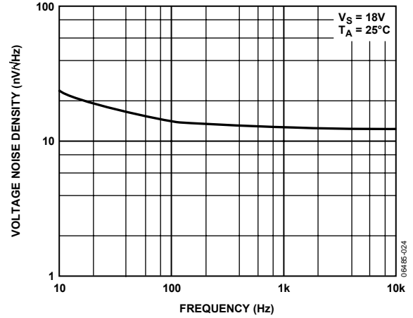
Figure 24. Voltage Noise Density vs. Frequency, V_S = 18V
