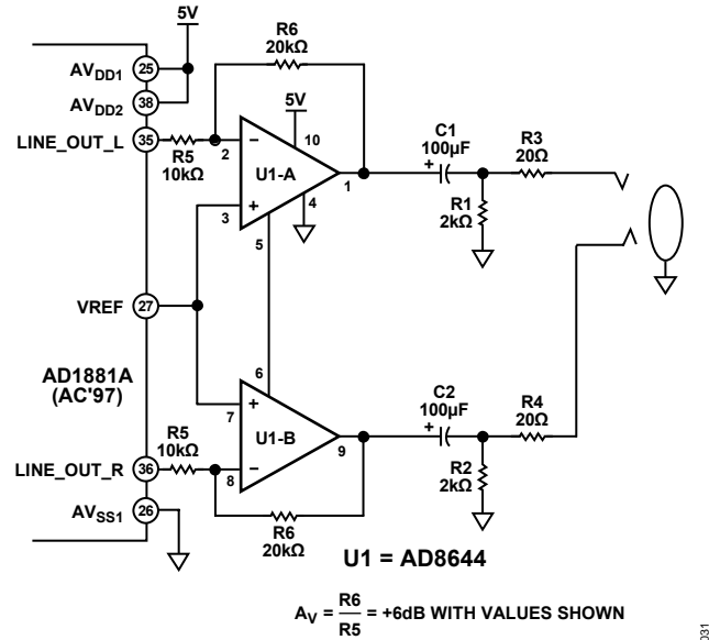
Figure 31. A PC-99-Compliant Headphone/Speaker Amplifier with Gain
