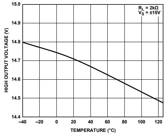
Figure 25. High Output Voltage, V_{OH} vs. Temperature, V_S = \pm 15\text{ V}
