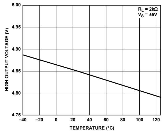
Figure 26. High Output Voltage, V_{OH} vs. Temperature, V_S = \pm 5\text{ V}
