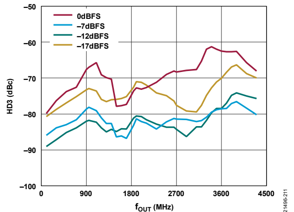
Figure 11. HD3 vs. f_{OUT} over Digital Scale, 9 GSPS DAC Sample Rate, Channel Interpolation 1x, Main Interpolation 6x, Mode 15C
