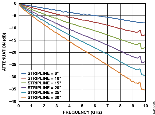
Figure 95. Insertion Loss of 50 Ω Striplines on FR4
