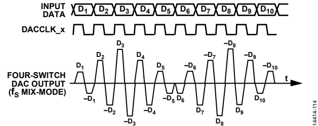
Figure 130. Mix-Mode Waveform
