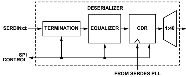
Figure 49. Deserializer Block Diagram
