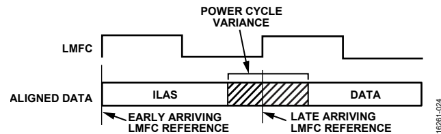
Figure 62. Link Delay > LMFC Period Example
