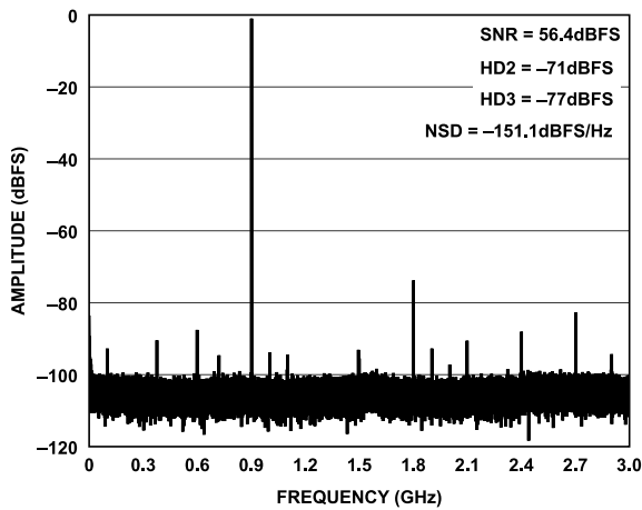
Figure 6. Single-Tone FFT at f_{IN} = 900 MHz
