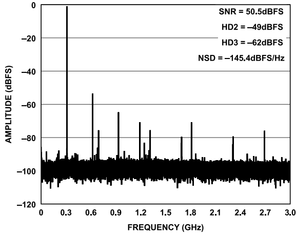
Figure 18. Single-Tone FFT at f_{IN} = 6.3 GHz
