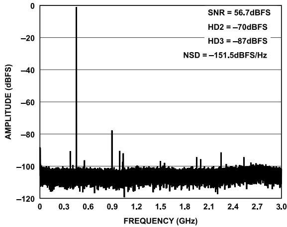
Figure 5. Single-Tone FFT at f_{IN} = 450 MHz
