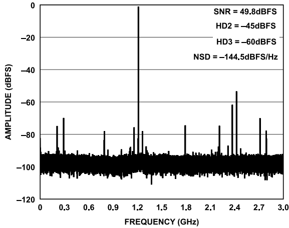
Figure 19. Single-Tone FFT at f_{IN} = 7.2 GHz
