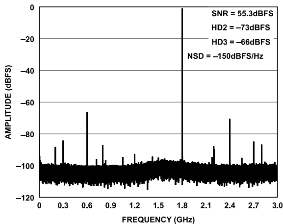
Figure 7. Single-Tone FFT at f_{IN} = 1.8 GHz
