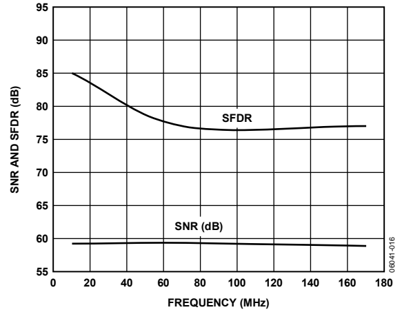
Figure 9. AD9211-200 Single-Tone SNR/SFDR vs. Input Frequency ( f_n ) with 1.25 V p-p Full Scale; 200 MSPS
