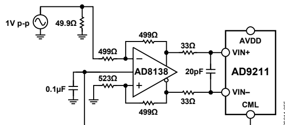
Figure 39. Differential Input Configuration Using the AD8138
