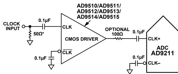
Figure 46. Single-Ended 3.3 V CMOS Sample Clock
