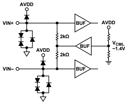
Figure 34. Analog Inputs ( V_{CML} \approx 1.4 V )
