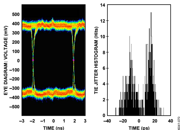
Figure 48. Data Eye for LVDS Outputs in ANSI Mode with Trace Lengths Less than 24 Inches on Standard FR-4, AD9211-250
