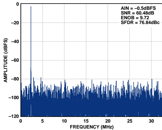
Figure 17. Single-Tone 32k FFT with f_{IN} = 2.3 MHz, AD9212-65
