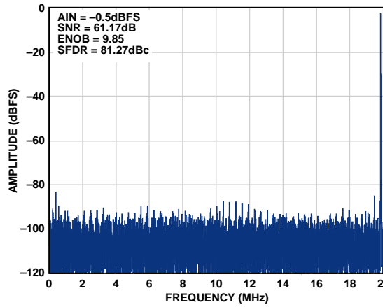
Figure 16. Single-Tone 32k FFT with f_{IN} = 19.7 MHz, AD9212-40
