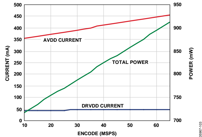
Figure 70. Supply Current vs. f_{SAMPLE} for f_{IN} = 10.3 MHz, AD9222- 65
