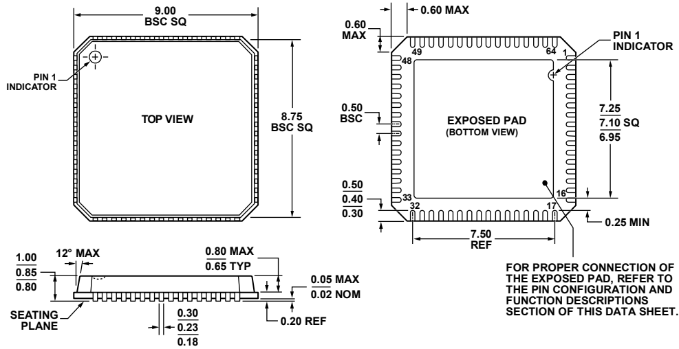
Figure 101. 64-Lead Lead Frame Chip Scale Package [LFCSP_VQ] 9 mm x 9 mm Body, Very Thin Quad (CP-64-3) Dimensions shown in millimeters
