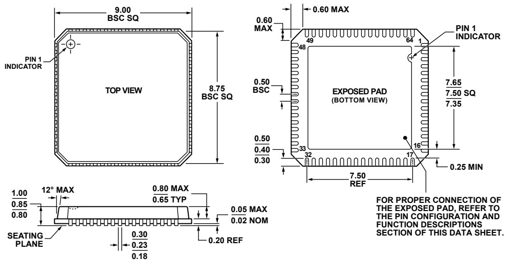
Figure 102. 64-Lead Lead Frame Chip Scale Package [LFCSP_VQ] 9 mm x 9 mm Body, Very Thin Quad (CP-64-6) Dimensions shown in millimeters
