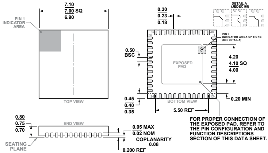
Figure 71. 48-Lead Lead Frame Chip Scale Package [LFCSP] 7 mm × 7 mm Body and 0.75 mm Package Height (CP-48-5)
