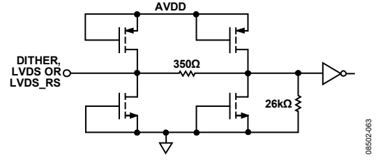
Figure 63. Equivalent DITHER, LVDS, and LVDS_RS Input Circuit
